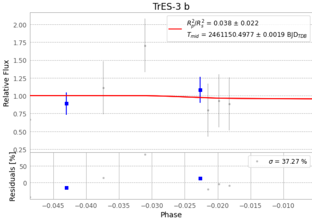
Figure 1 — FinalLightCurve_TrES-3 b_2026-04-20.png (SHA-256 145c3d7a786cac74...)
