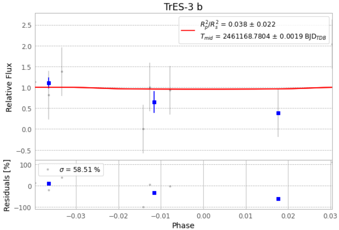
Figure 1 — FinalLightCurve_TrES-3 b_2026-05-07.png (SHA-256 5c455738bb148801...)
