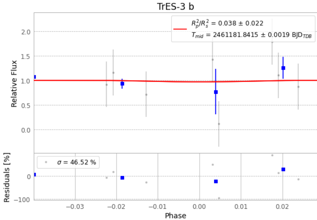
Figure 1 — FinalLightCurve_TrES-3 b_2026-05-21.png (SHA-256 a7423b264d9b8e97...)
