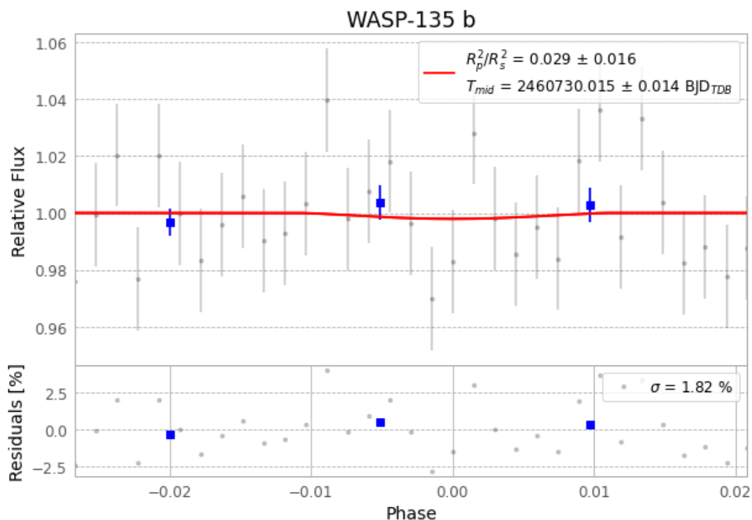
Figure 1 — FinalLightCurve_WASP-135 b_2025-02-23.png (SHA-256 5b1e54e94a216897...)
