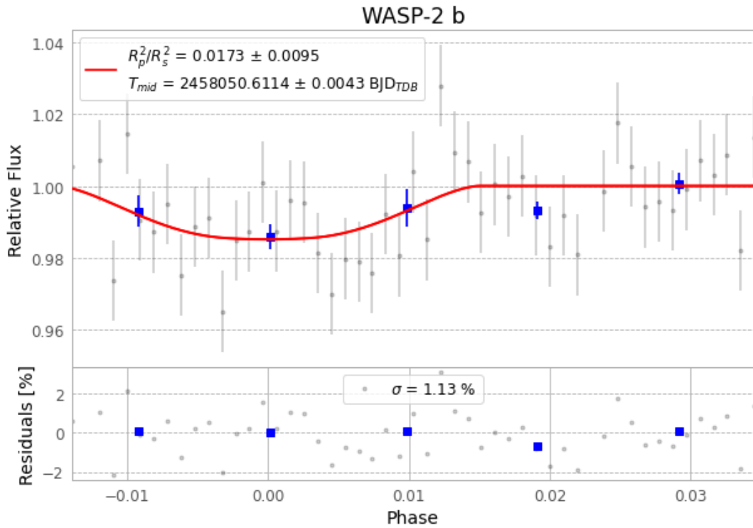
Figure 1 — FinalLightCurve_WASP-2 b_2017-10-23.png (SHA-256 0c77ad2b2dd1ec4b...)
