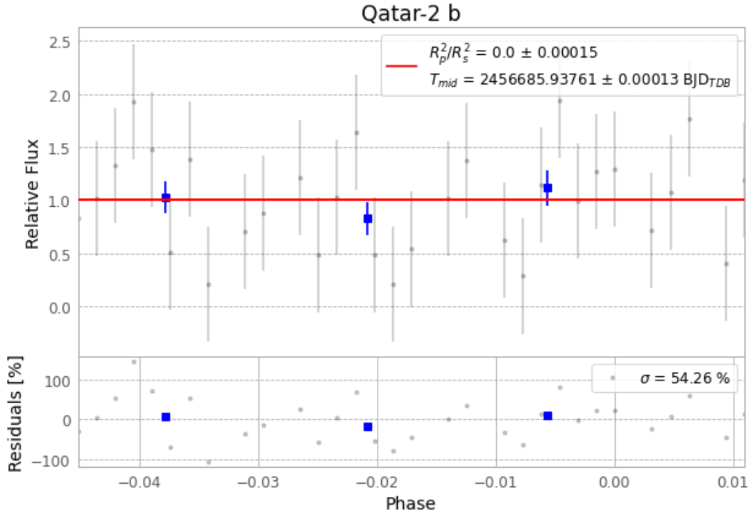
Figure 1 — FinalLightCurve_Qatar-2 b_2014-01-28.png (SHA-256 5738e941d3af674c...)
