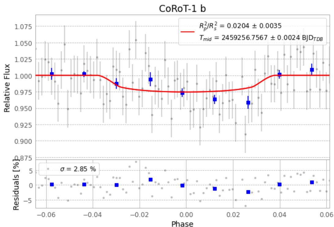
Figure 1 — FinalLightCurve_CoRoT-1 b_2021-02-10.png (SHA-256 8d26e2bc3ab3b7da...)
