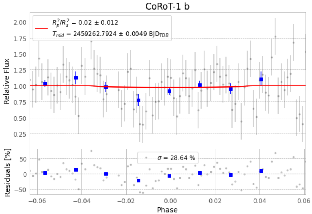
Figure 1 — FinalLightCurve_CoRoT-1 b_2021-02-16.png (SHA-256 33b28043921a5451...)
