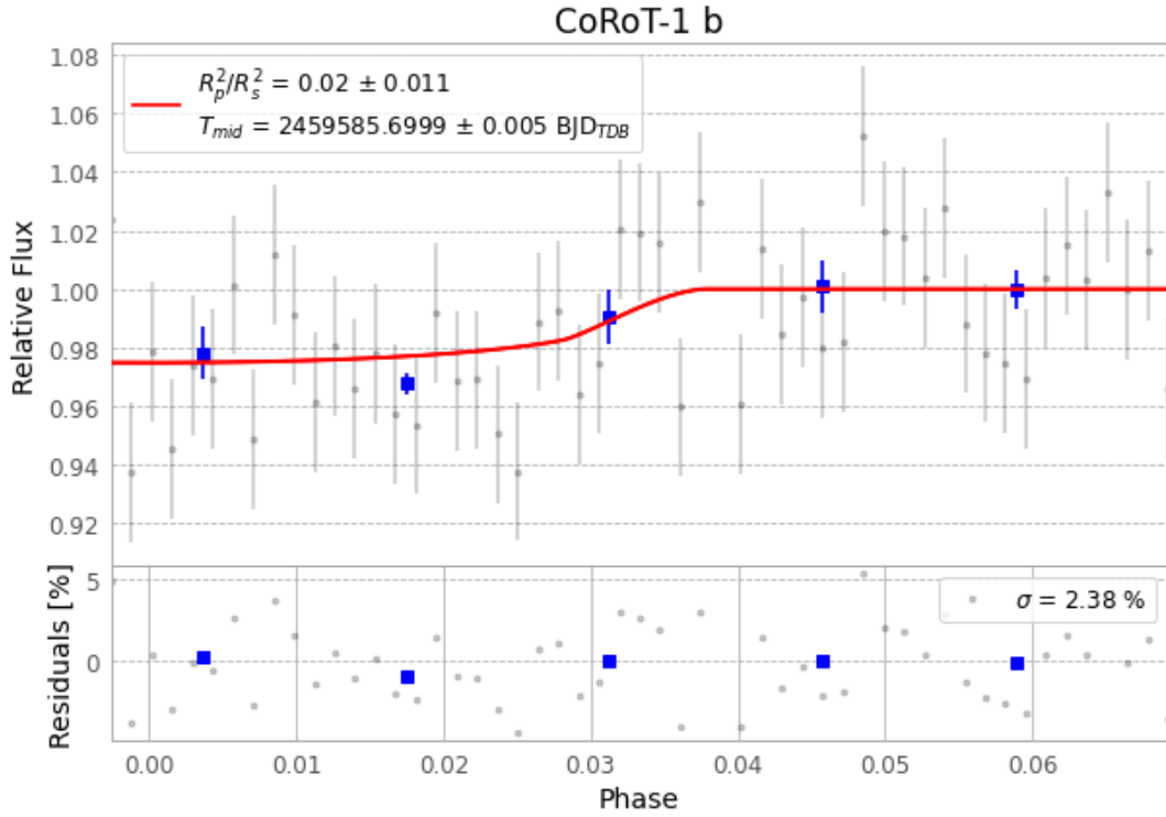
Figure 1 — FinalLightCurve_CoRoT-1 b_2022-01-05.png (SHA-256 21ea857bf336f332...)
