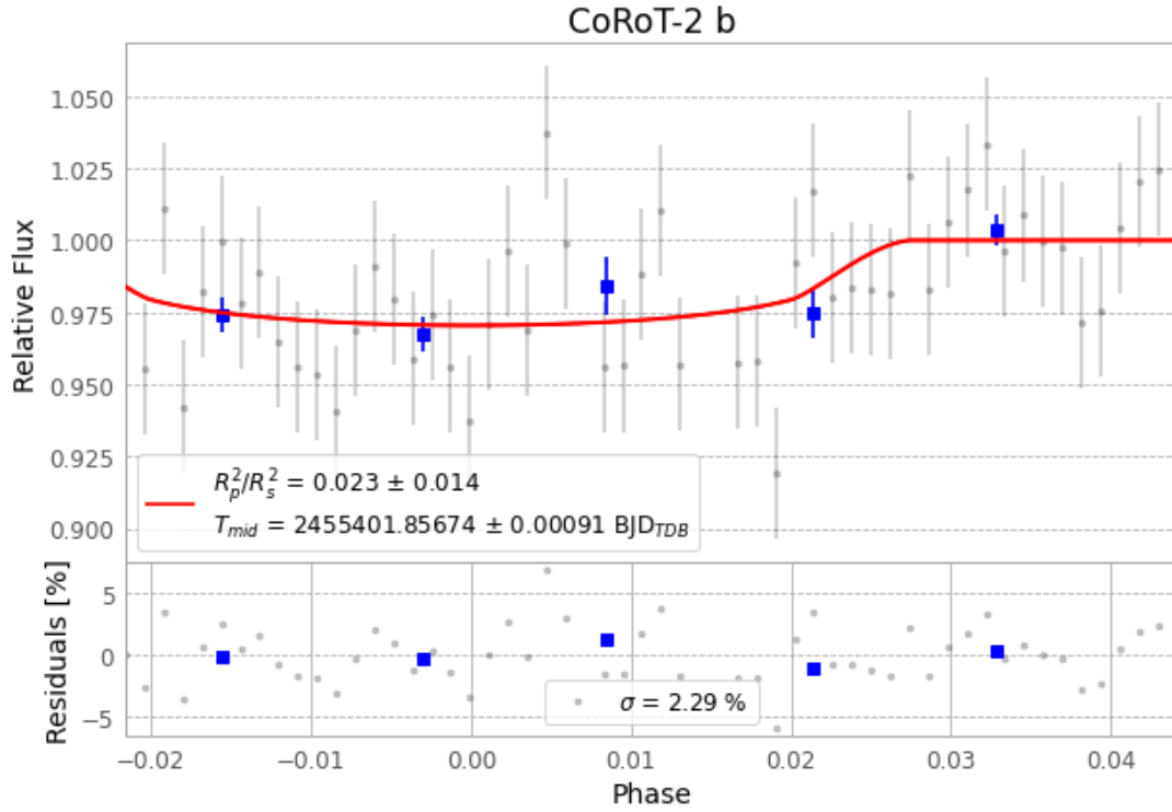
Figure 1 — FinalLightCurve_CoRoT-2 b_2010-07-24.png (SHA-256 Oddadf1ee5c1bbd1...)
