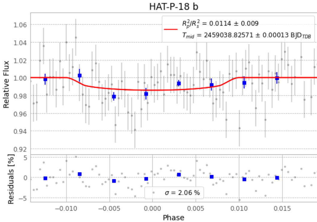
Figure 1 — FinalLightCurve_HAT-P-18 b_2020-07-07.png (SHA-256 41e6dc0ed5313de4...)
