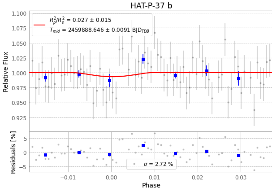
Figure 1 — FinalLightCurve_HAT-P-37 b_2022-11-04.png (SHA-256 b53db65d06165edf...)
