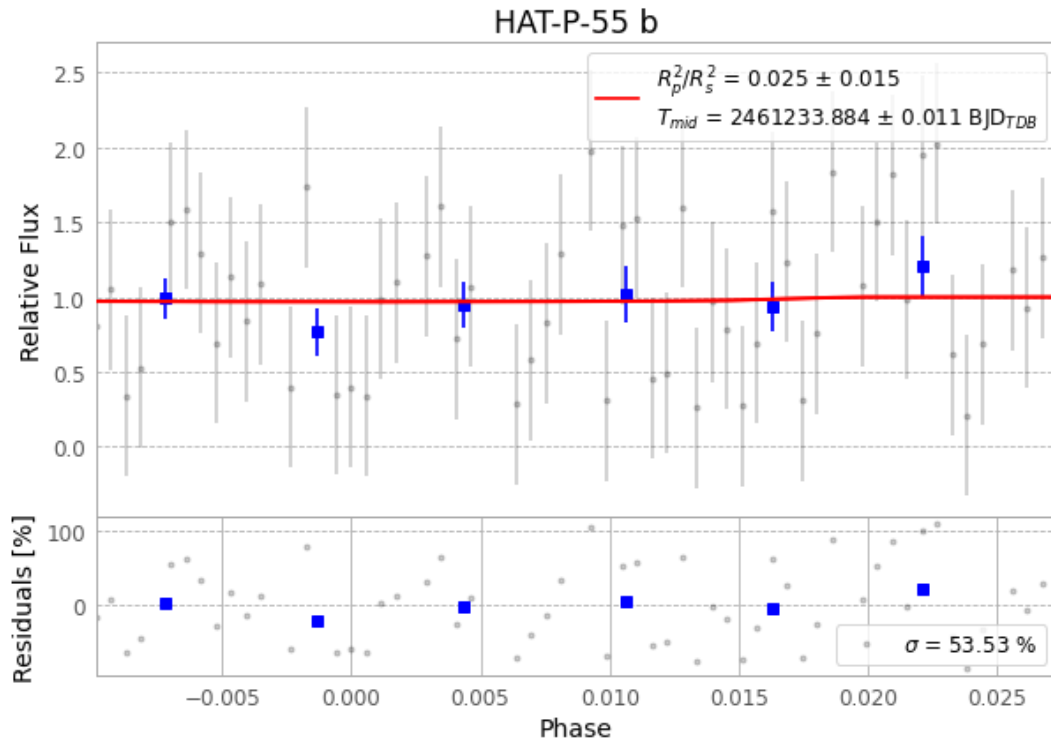
Figure 1 — FinalLightCurve_HAT-P-55 b_2026-07-12.png (SHA-256 4edf42c4346b49c8...)
