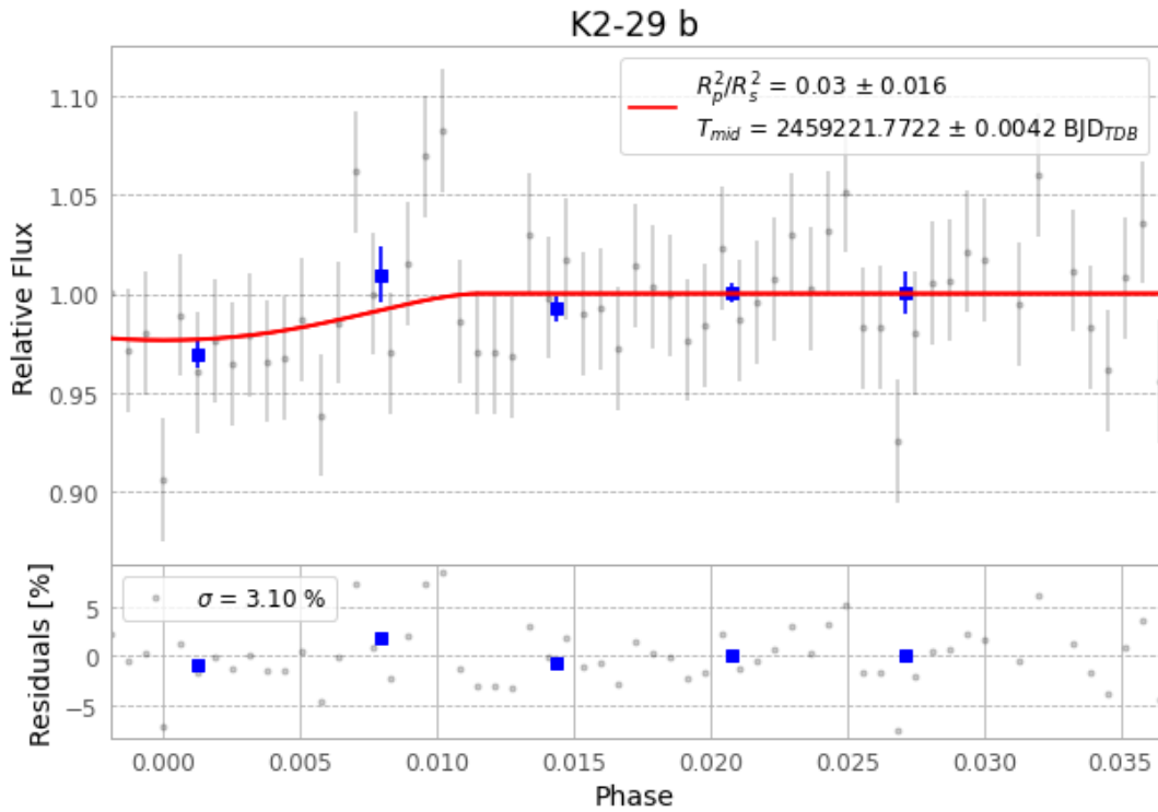
Figure 1 — FinalLightCurve_K2-29 b_2021-01-06.png (SHA-256 f09baec967aeb3f6...)
