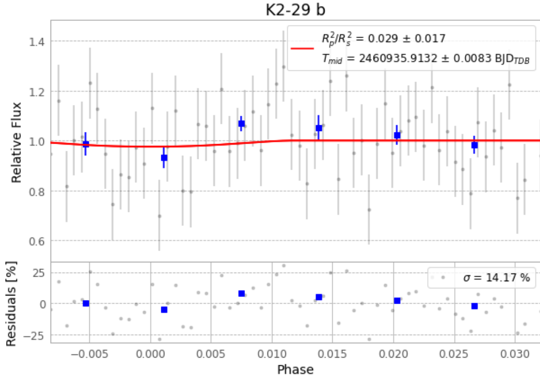
Figure 1 — FinalLightCurve_K2-29 b_2025-09-17.png (SHA-256 f558aaabd09716f8...)
