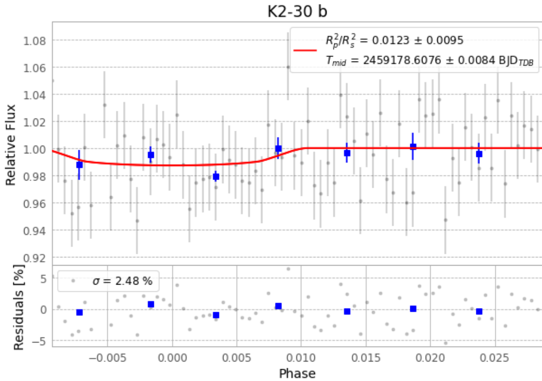
Figure 1 — FinalLightCurve_K2-30 b_2020-11-24.png (SHA-256 c18c81ec2af84ae8...)
