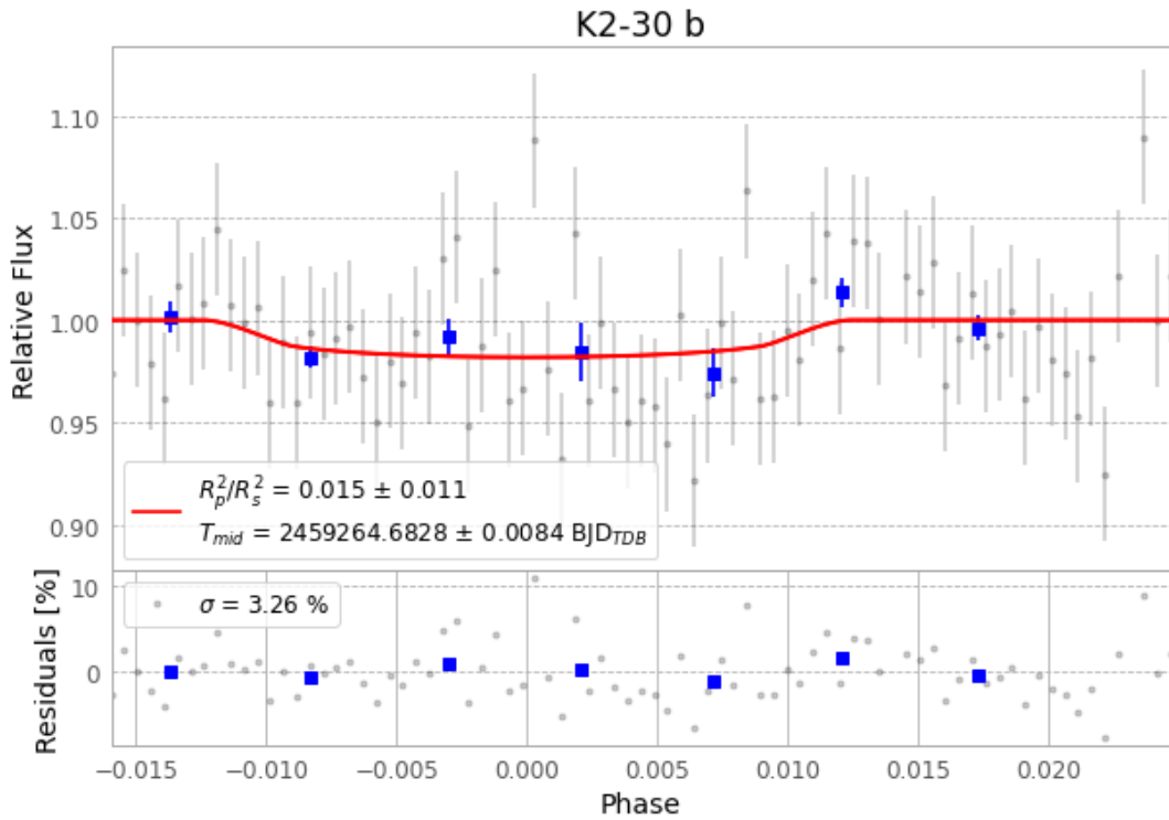
Figure 1 — FinalLightCurve_K2-30 b_2021-02-18.png (SHA-256 2ad1ee5596431c28...)
