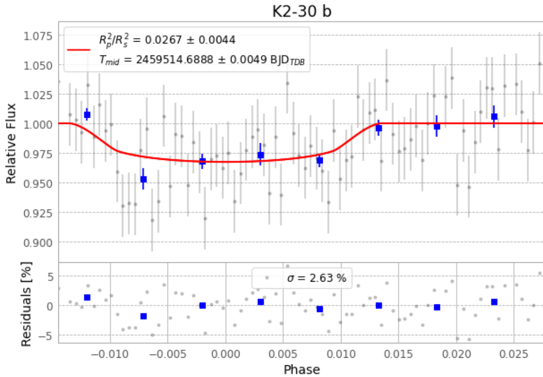
Figure 1 — FinalLightCurve_K2-30 b_2021-10-26.png (SHA-256 c3b0efd9a5ba943c...)
