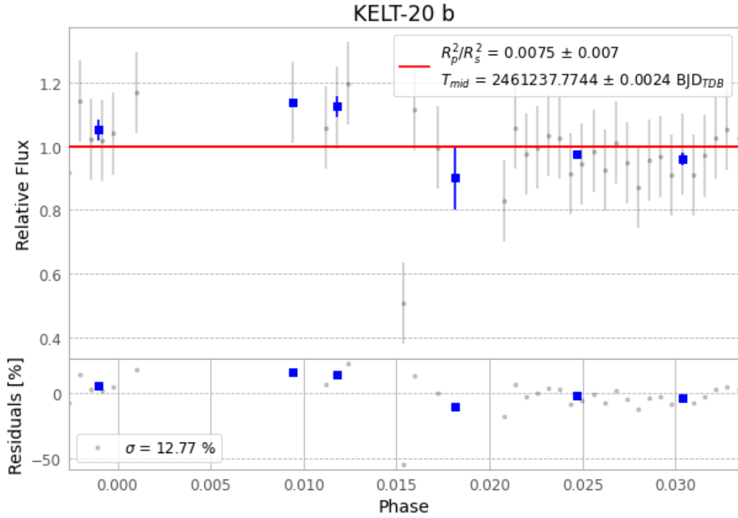
Figure 1 — FinalLightCurve_KELT-20 b_2026-07-15.png (SHA-256 0b2540d51b1742ef...)
