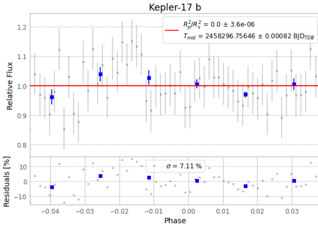
Figure 1 — FinalLightCurve_Kepler-17 b_2018-06-26.png (SHA-256 6ccdb9bdc8cc35ae...)
