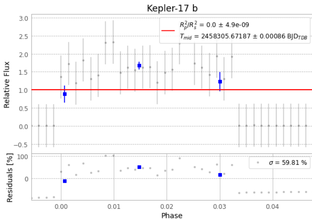
Figure 1 — FinalLightCurve_Kepler-17 b_2018-07-05.png (SHA-256 d0e73e9c07cfc932...)
