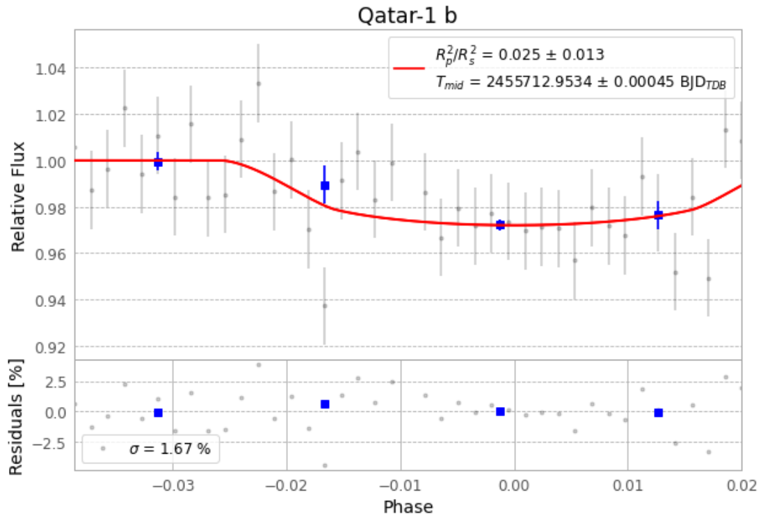
Figure 1 — FinalLightCurve_Qatar-1 b_2011-05-31.png (SHA-256 8ac2a7d855fce630...)
