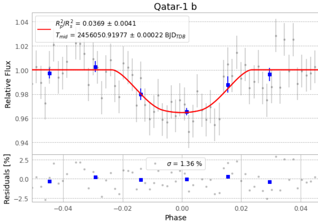
Figure 1 — FinalLightCurve_Qatar-1 b_2012-05-03.png (SHA-256 9691ec92dd348615...)
