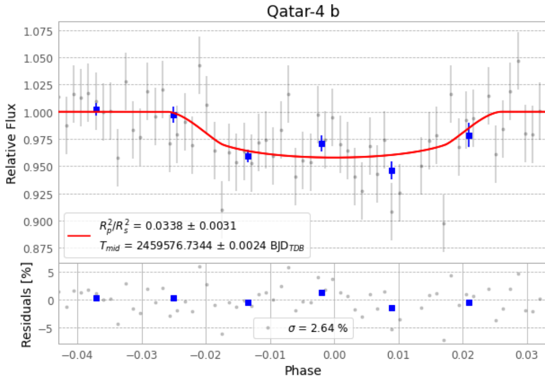
Figure 1 — FinalLightCurve_Qatar-4 b_2021-12-27.png (SHA-256 de79690d6c45c9c3...)
