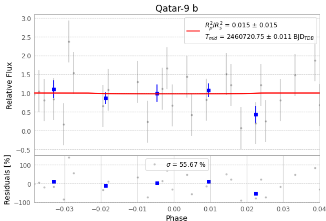
Figure 1 — FinalLightCurve_Qatar-9 b_2025-02-13.png (SHA-256 dbd447c2e4bd1293...)
