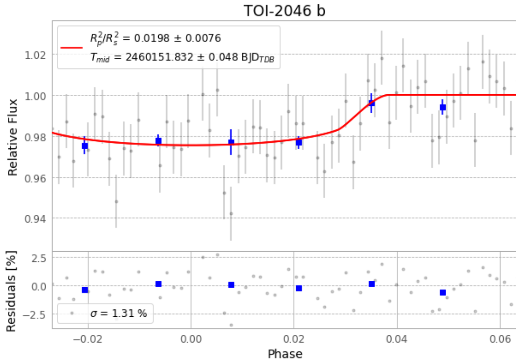
Figure 1 — FinalLightCurve_TOI-2046 b_2023-07-26.png (SHA-256 00037f511bfa588b...)
