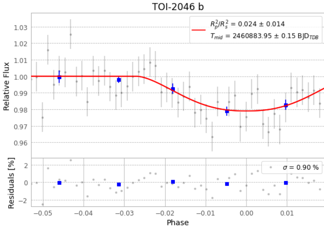
Figure 1 — FinalLightCurve_TOI-2046 b_2025-07-27.png (SHA-256 02104c01823a5a29...)
