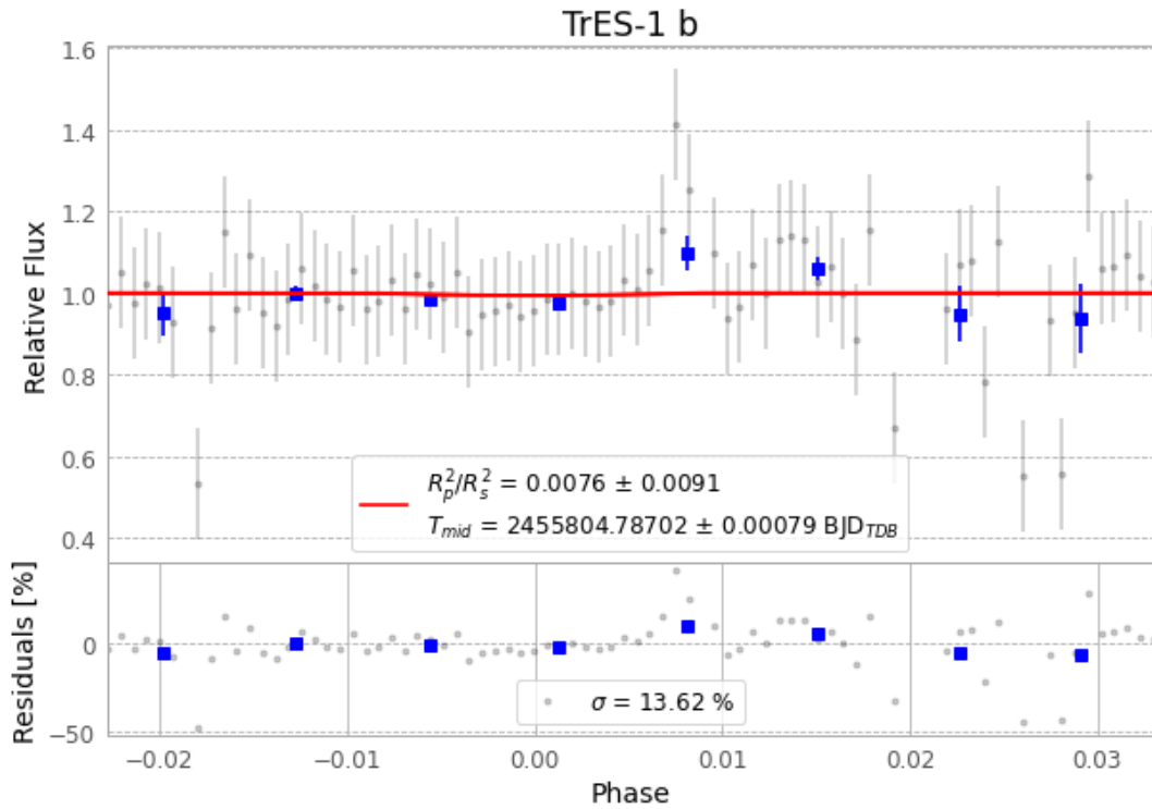
Figure 1 — FinalLightCurve_TrES-1 b_2011-08-30.png (SHA-256 6b763daeac892a30...)
