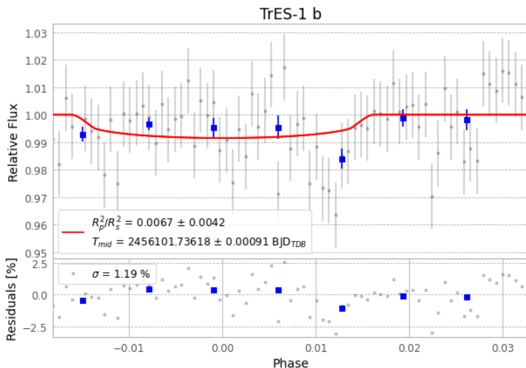
Figure 1 — FinalLightCurve_TrES-1 b_2012-06-22.png (SHA-256 478d108767097c0a...)
