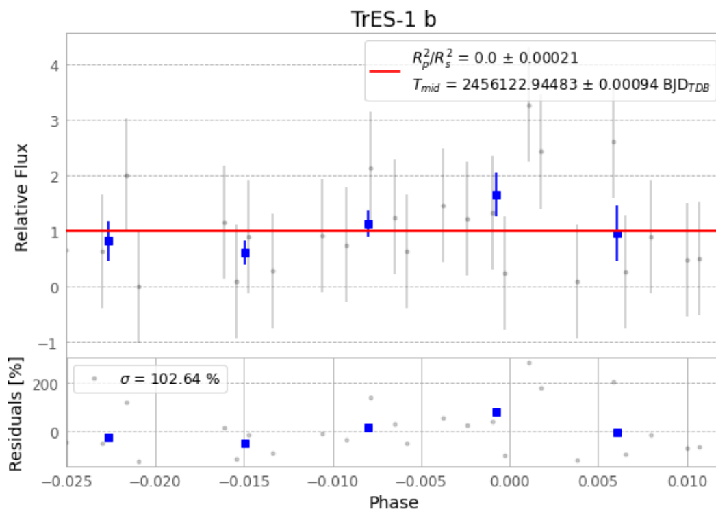
Figure 1 — FinalLightCurve_TrES-1 b_2012-07-14.png (SHA-256 46a065690c581901...)
