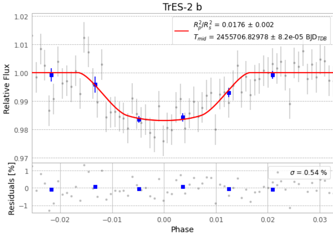
Figure 1 — FinalLightCurve_TrES-2 b_2011-05-24.png (SHA-256 9e6f04bba1a2feb1...)
