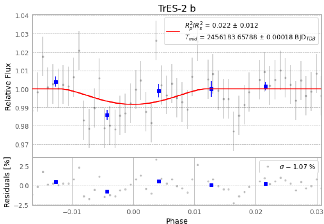
Figure 1 — FinalLightCurve_TrES-2 b_2012-09-12.png (SHA-256 9e7e904de1f14ff4...)
