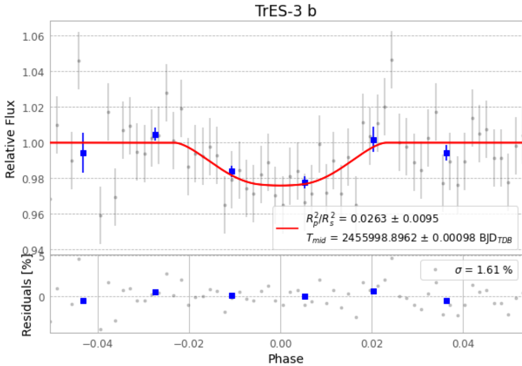
Figure 1 — FinalLightCurve_TrES-3 b_2012-03-12.png (SHA-256 2e2ddf195efa73ef...)
