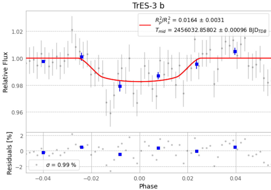
Figure 1 — FinalLightCurve_TrES-3 b_2012-04-15.png (SHA-256 e12a89a02d1b7a0e...)
