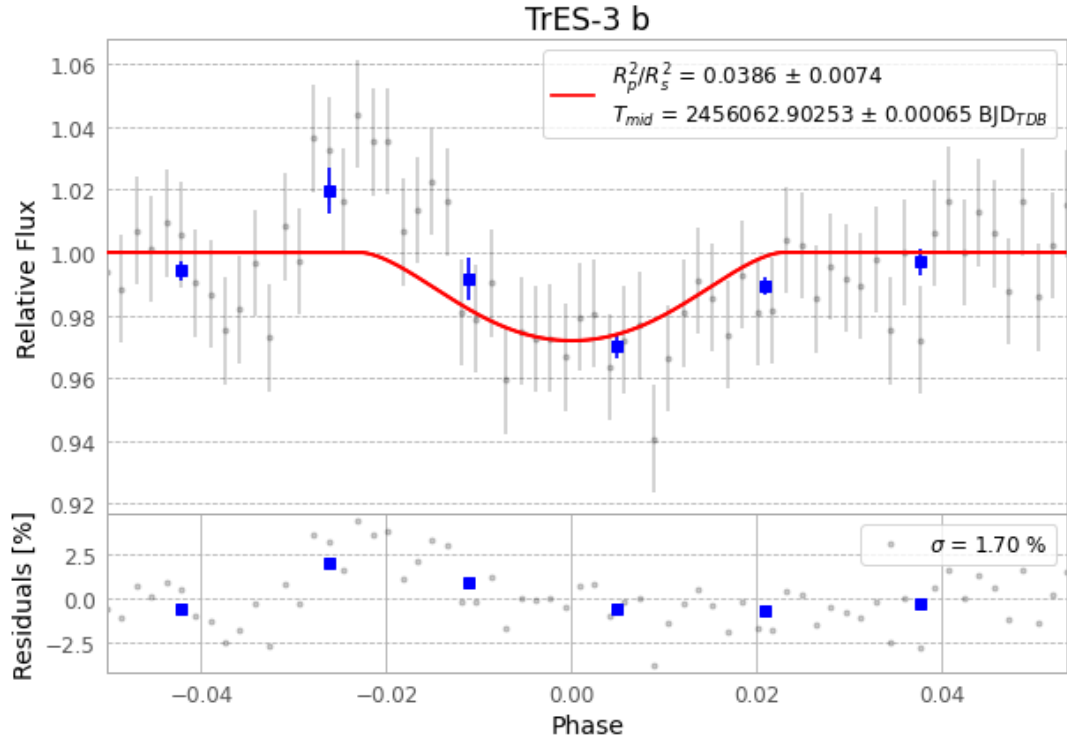
Figure 1 — FinalLightCurve_TrES-3 b_2012-05-15.png (SHA-256 5548d898552b1386...)
