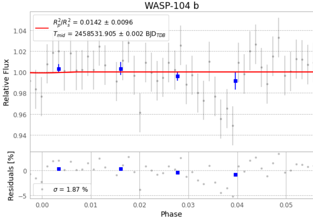
Figure 1 — FinalLightCurve_WASP-104 b_2019-02-17.png (SHA-256 04c9ae9bc3618793...)
