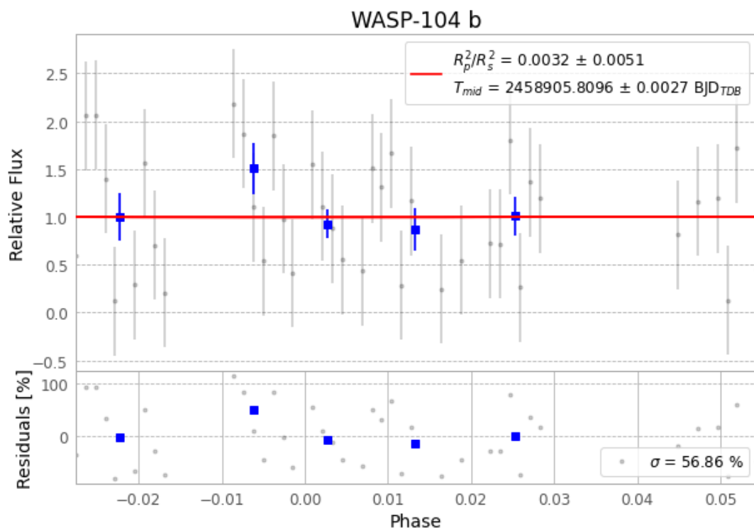
Figure 1 — FinalLightCurve_WASP-104 b_2020-02-25.png (SHA-256 2d4b55d94a528536...)
