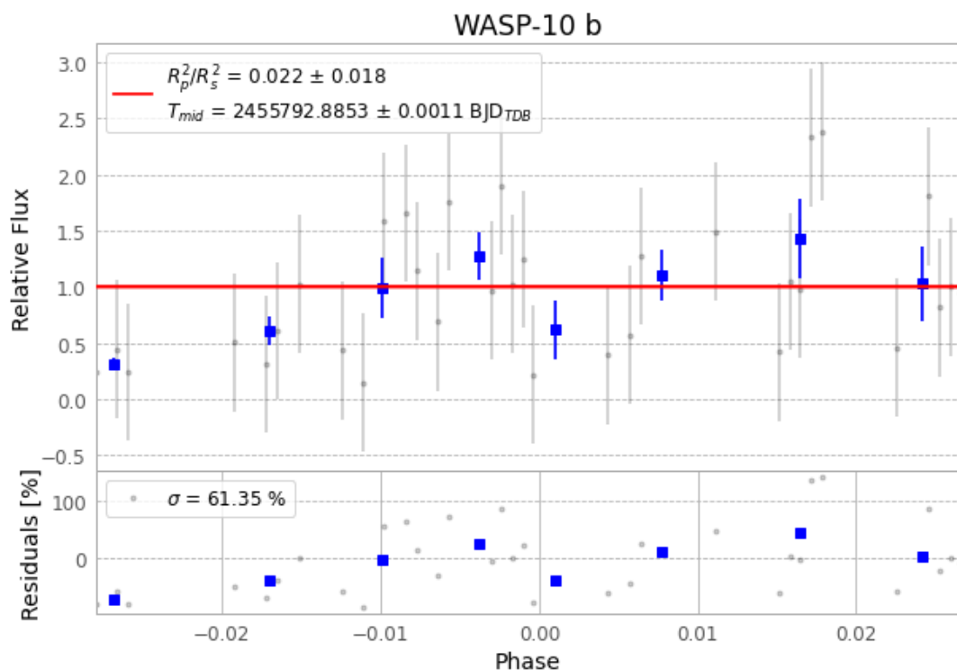
Figure 1 — FinalLightCurve_WASP-10 b_2011-08-19.png (SHA-256 864b09186988f6d5...)
