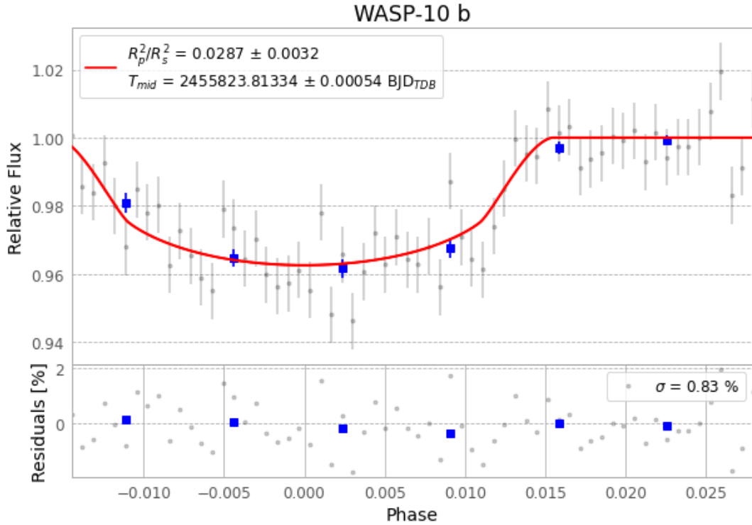
Figure 1 — FinalLightCurve_WASP-10 b_2011-09-18.png (SHA-256 a336b9b2932c009b...)
