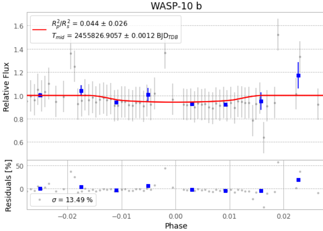
Figure 1 — FinalLightCurve_WASP-10 b_2011-09-22.png (SHA-256 3364ee2ce4dda078...)
