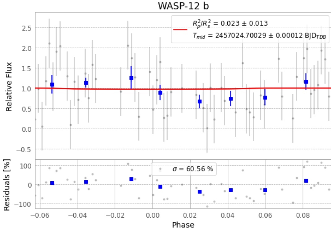
Figure 1 — FinalLightCurve_WASP-12 b_2015-01-01.png (SHA-256 74e9ea6e1f3453b9...)
