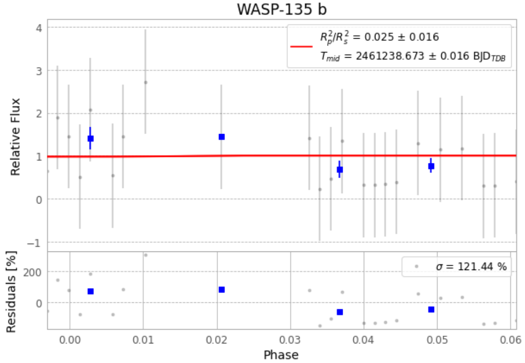
Figure 1 — FinalLightCurve_WASP-135 b_2026-07-16.png (SHA-256 b5bb0f0aad6b0b7d...)
