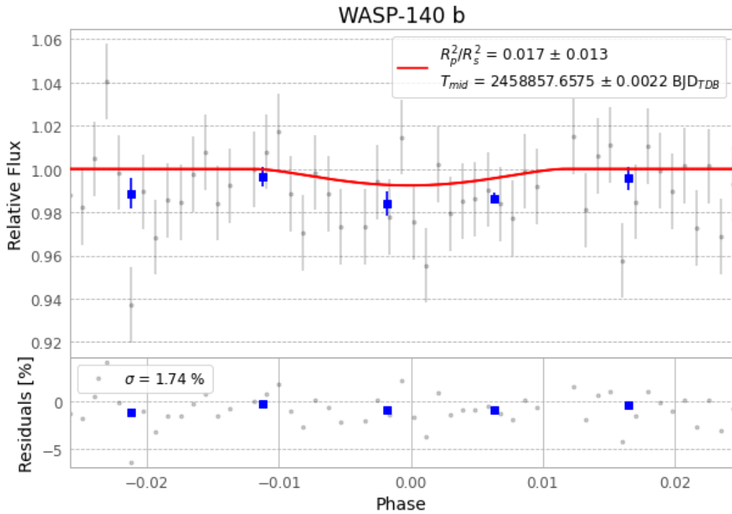
Figure 1 — FinalLightCurve_WASP-140 b_2020-01-08.png (SHA-256 541cd6e523b487b8...)
