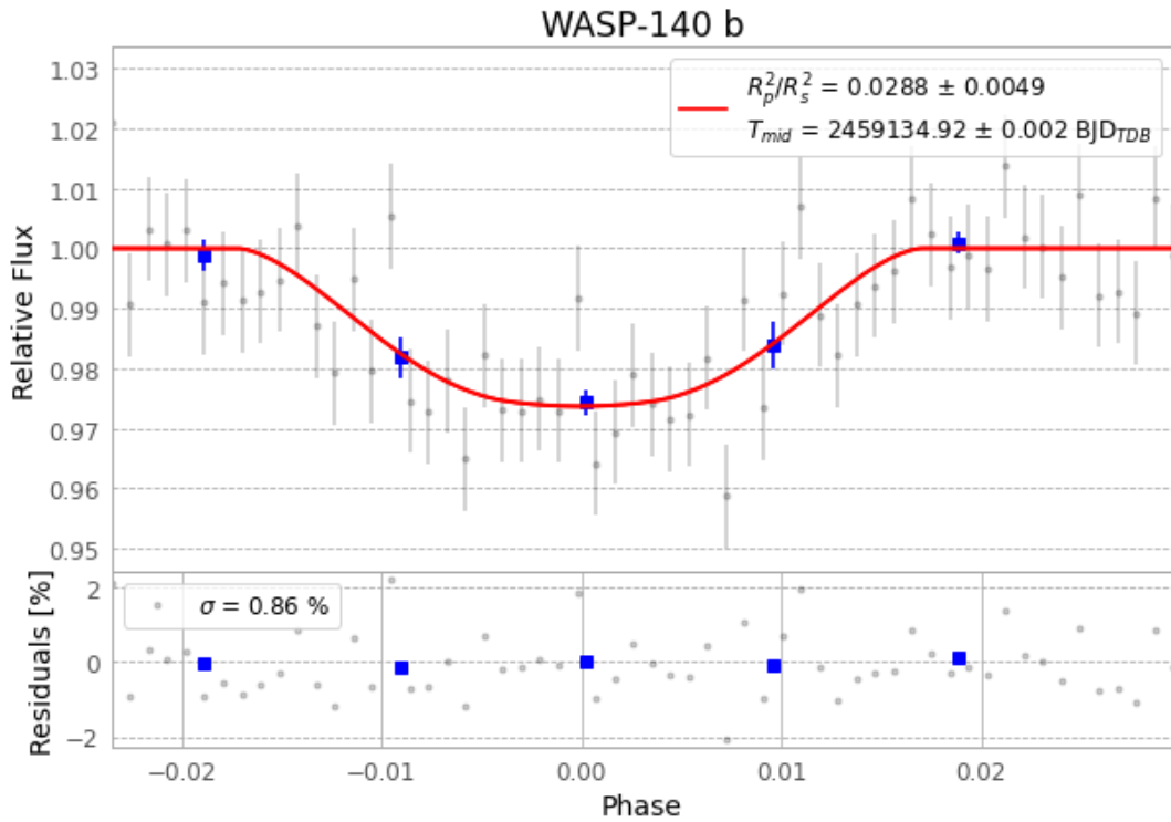
Figure 1 — FinalLightCurve_WASP-140 b_2020-10-12.png (SHA-256 24440e5b25106e96...)
