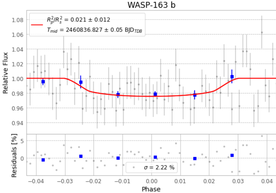
Figure 1 — FinalLightCurve_WASP-163 b_2025-06-09.png (SHA-256 b376e61388a93ef9...)
