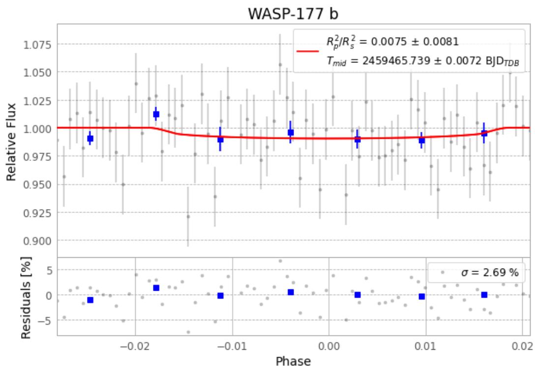
Figure 1 — FinalLightCurve_WASP-177 b_2021-09-07.png (SHA-256 3f6fc5438392b3c8...)
