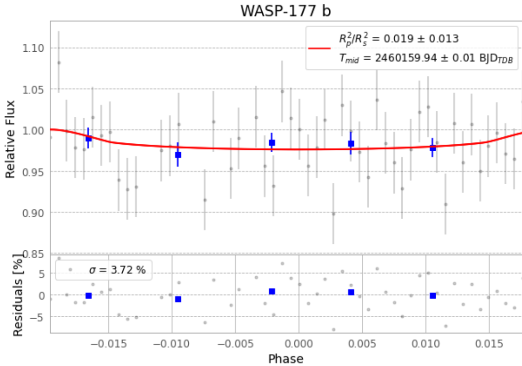
Figure 1 — FinalLightCurve_WASP-177 b_2023-08-03.png (SHA-256 607963a3882f4806...)
