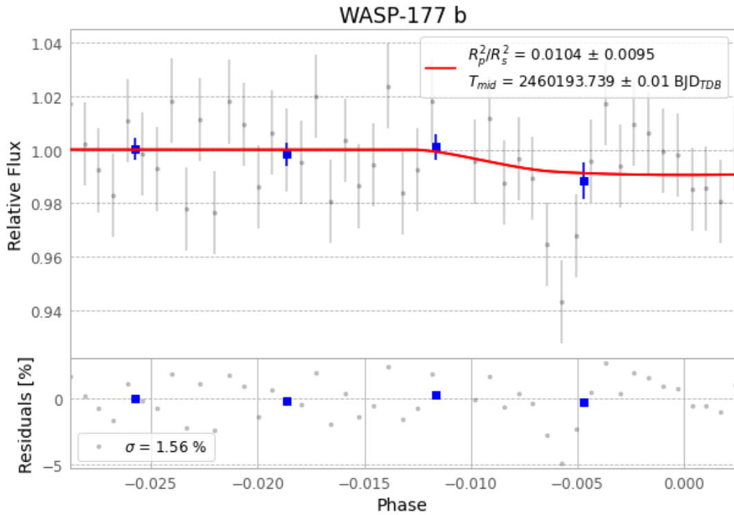
Figure 1 — FinalLightCurve_WASP-177 b_2023-09-05.png (SHA-256 9b230dba16473c5d...)
