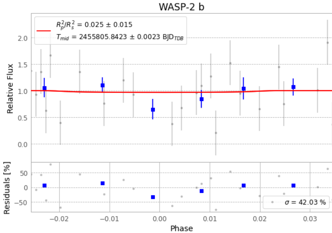
Figure 1 — FinalLightCurve_WASP-2 b_2011-08-31.png (SHA-256 850228065e4d8adb...)
