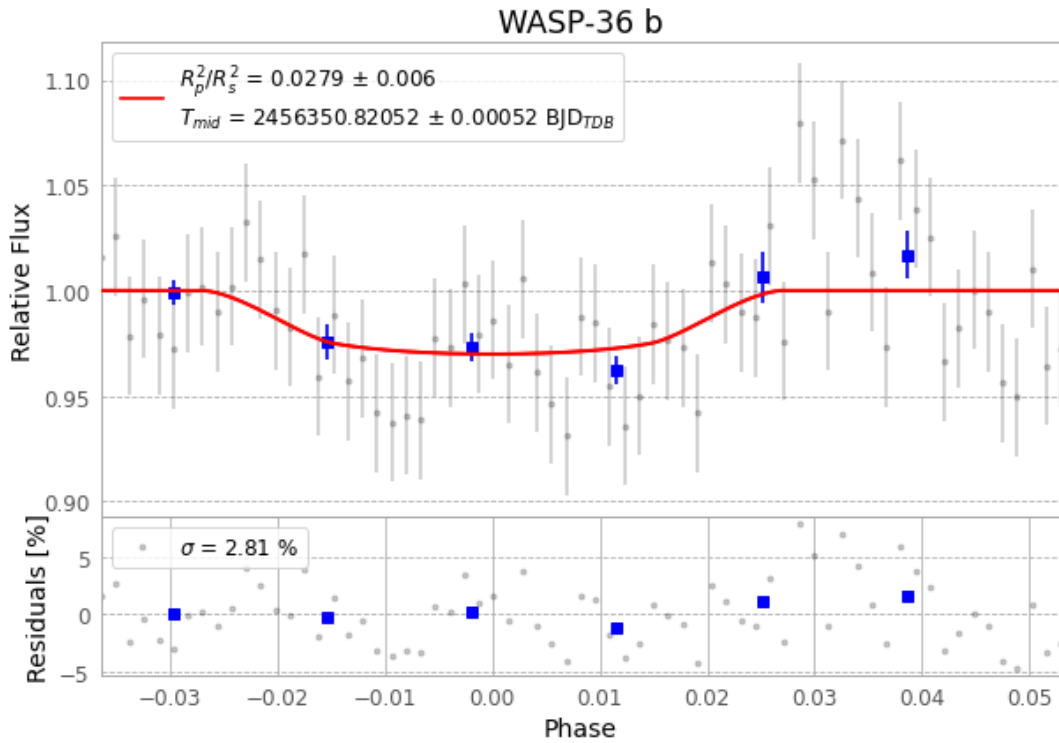
Figure 1 — FinalLightCurve_WASP-36 b_2013-02-26.png (SHA-256 003d69fd2a808410...)
